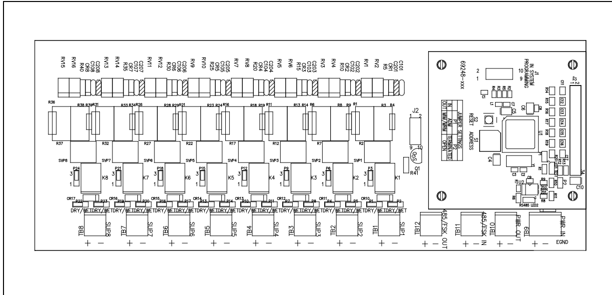
Figure 1. Model 12578-002 Monitored Input Module
